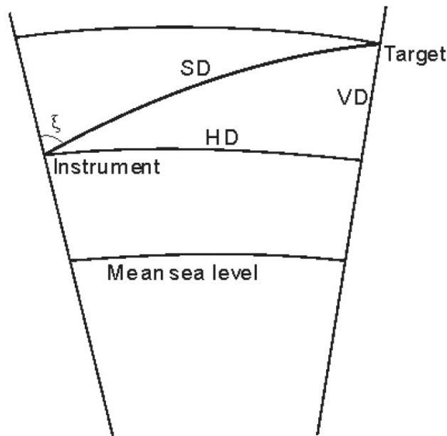
Elevation measurement
